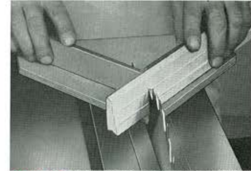
MITRE JIG most essential for accurate mitreing. Addition of bevelled strip permits compound angles to be cut.
