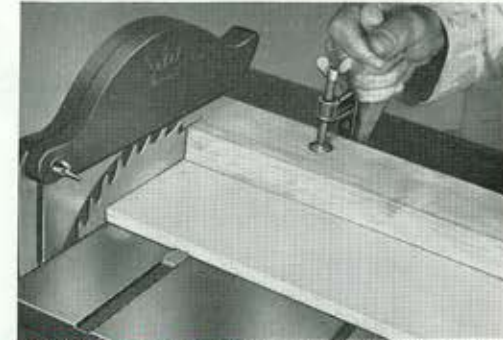
CROSS CUTTING JIG simplifies repetition cross cutting. Adjustable stop permits cutting of definite lengths.
