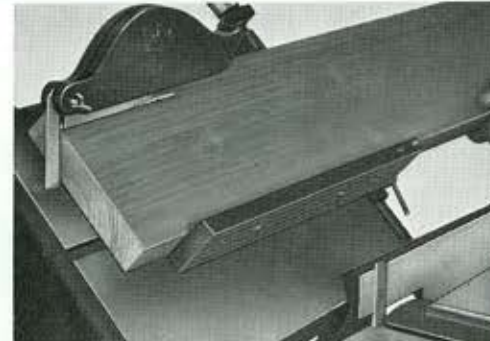
ANGLE SAWING up to 45° with table tilting on heavy graduated quadrant. Note guard and splitter (to prevent binding).
