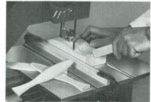
Pad cutting to produce multiples of same shape. Gives wide scope for repetition work.
