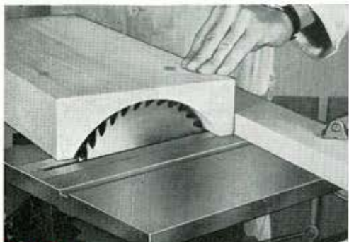
COVING with standard saw blade and wooden fence. Angle and placing of fence determines width and shape of cove. (Lower table approximately ½" per pass.)
