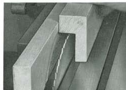
REBATING. Using false wooden fence to allow clean cut to edge of work. Wobble saw cuts up to \frac{1}{2} " wide by 2" deep at one pass for speedy production.
