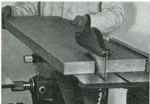
RIPSAWING 2" x 14" Oak board. Hard and softwoods handled with ease (see corner illustrations for capacities).
