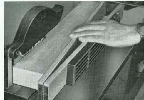
TAPERED RIP SAWING using simple hinged jig. Compound tapers can also be cut by tilting table. Useful when false cooping.
