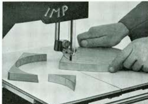
Accurate cutting of 7" circle in 1/2" aluminium using false table and jig, cutting time 4 minutes.
