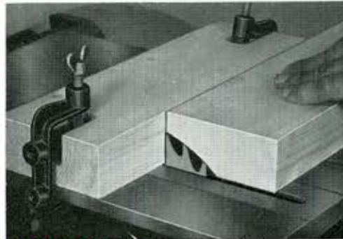
CORNER COVING. Using false wooden fence positioned to use portion of saw blade only. Increase cut by approximately ¼" each pass.
