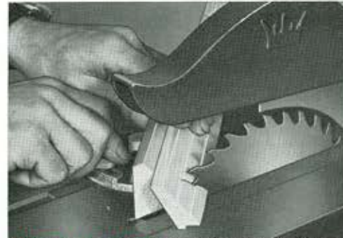
COMPOUND MITRES. Easily cut using bevelled strip fastened to mitre fence. Fence graduated to 60° either way.
