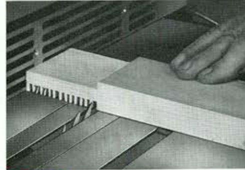
TENONING with series of cuts. Short ends break off easily, and finished with repeated cross movements. Thickened timbers ensure accuracy with this method.
